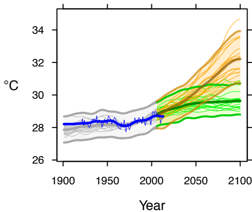
Fig 1.1. Under a high emissions scenario, mean annual temperature is projected to rise by about 3.8°C on average from 1990 to 2100. If global emissions decrease rapidly, the temperature rise is limited to about 1.2°C.
